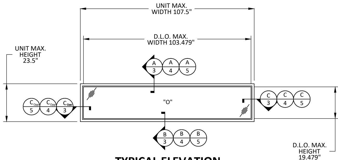
TYPICAL ELEVATION 800 DOOR TRANSOM
